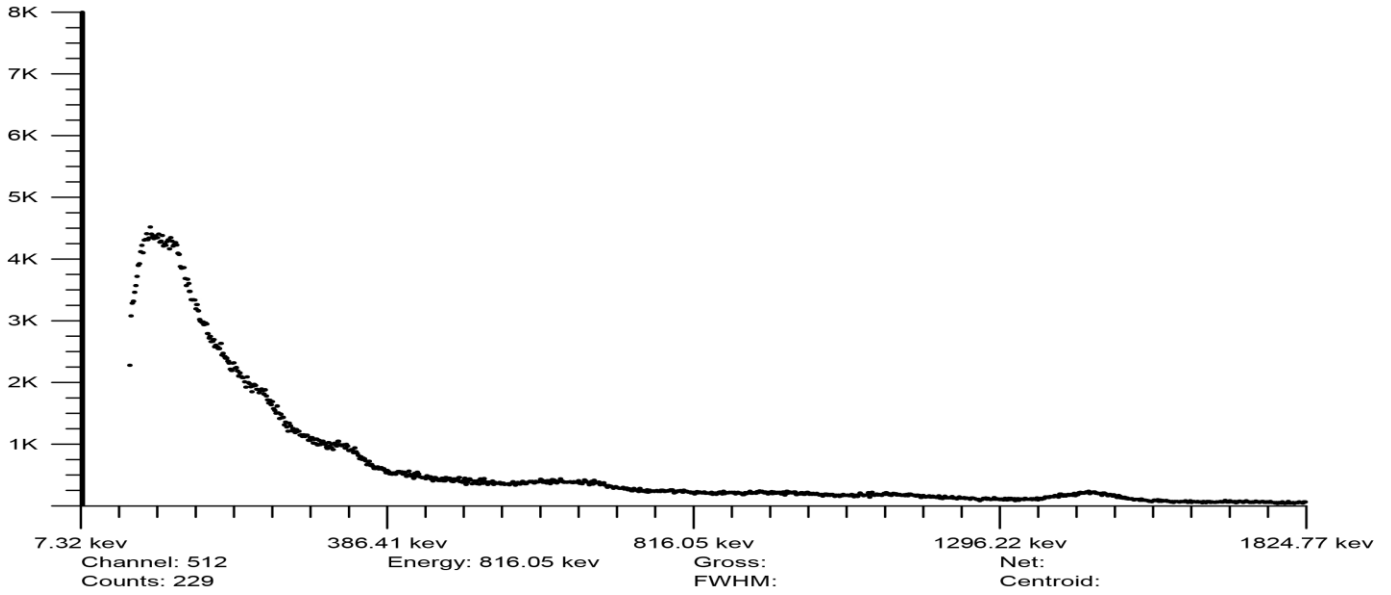
Fig. (4): Laboratory BG spectrum measured by NaI (Tl) detector.
