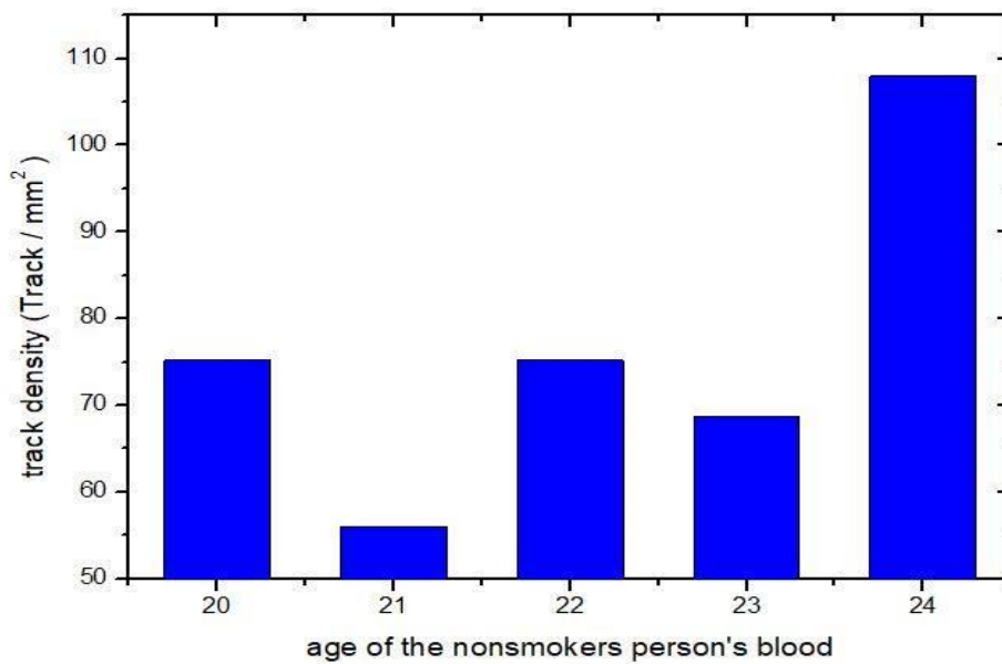
Figure 1: alpha particles density in the nonsmoker person's blood
