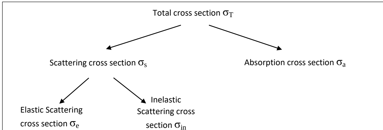
Schematic diagram of the Neutron cross section
