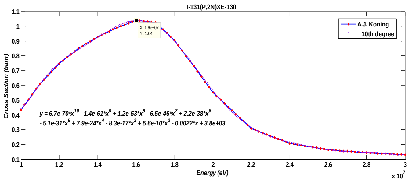
Fig.(1): The cross section of I-131(p,2n)Xe-130 as a function of Proton energy
